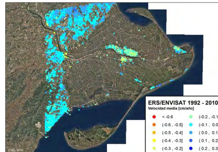
Vertical movements over Ebro Delta plain, measured through ERS and ENVISAT imagery. Negative values indicate subsidence
